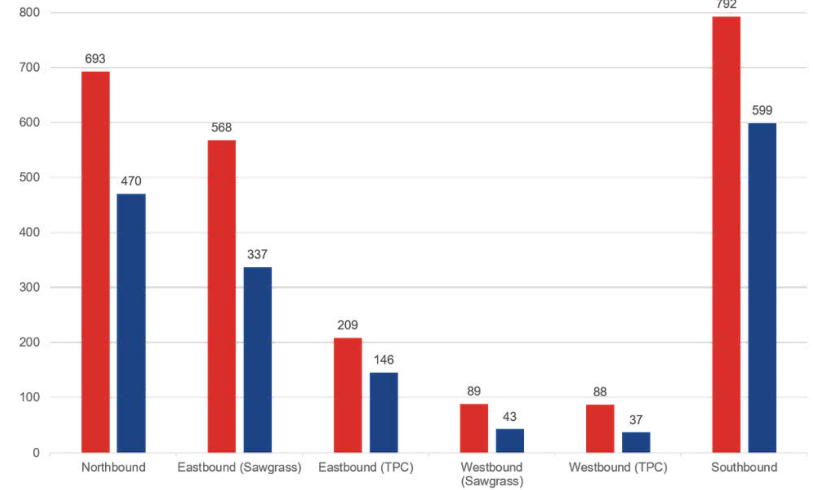
PM Peak Hour - Queue Length (feet)
