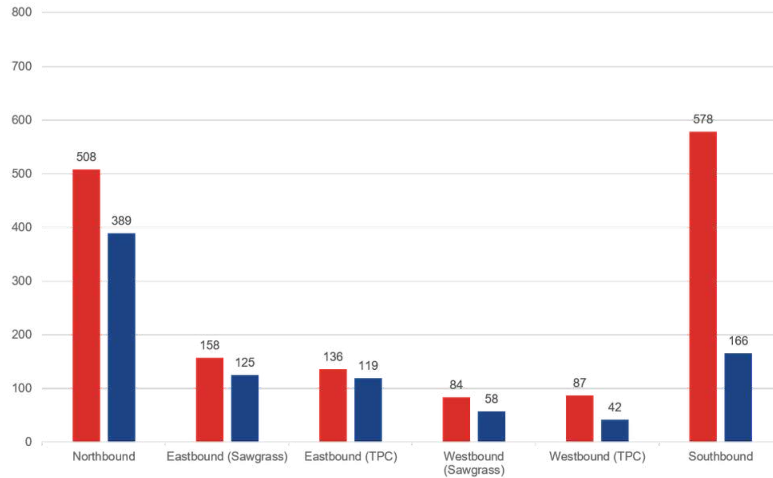
AM Peak Hour - Queue Length (feet)
